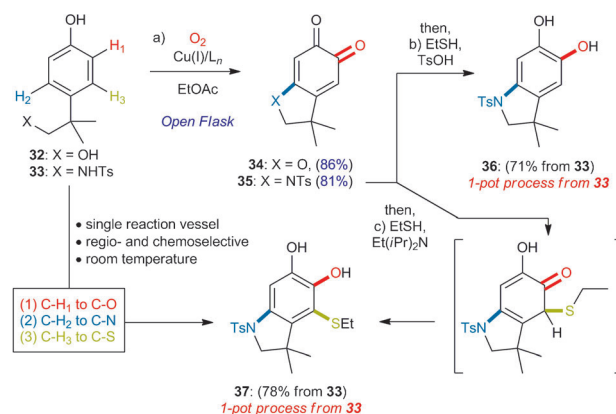
Scheme 3. Cross-aerobic coupling. Reagents and conditions: a) Synthesis of 34 and 35 : 3 (4 mol %), DBED (5 mol %), EtOAc (0.5 M), open flask. Synthesis of 36 from 33 : 3 (4 mol %), DBED (5 mol %), CH 2 Cl 2 (0.1 M), O 2 (1 atm); then EtSH (4 equiv), para -toluenesulfonic acid (1 equiv). Synthesis of 37 : 3 (4 mol %), DBED (5 mol %), CH 2 Cl 2 (0.1 M), O 2 (1 atm); then EtSH (4 equiv), DBED (1 equiv).
