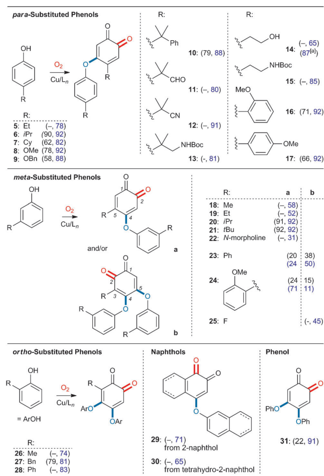
Scheme 2. Substrate scope. Standard Et 3 N conditions (isolated yields of products are shown first, in black): phenol (1.0 mmol), O 2 (1 atm), 3 (8 mol %), Et 3 N (50 mol %), 4 Å molecular sieves (200 mg), CH 2 Cl 2 (0.1 M) at 25 °C for 4 h. Standard DBED conditions (isolated yields of products are shown second, in blue): phenol (1.0 mmol), O 2 (1 atm), 3 (4 mol %), DBED (5 mol %), CH 2 Cl 2 (0.1–0.5 M) at 23 °C for 4 h. [a] Reaction performed in THF (0.1 M) because of issues of solubility.
