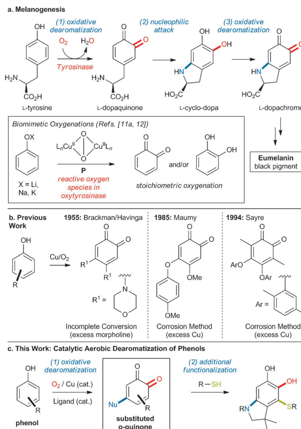
Scheme 1. a) Principle steps of melanogenesis leading to eumelanin and the reactive oxygen species of the enzyme tyrosinase. b) Previous examples of phenolic oxygenation/functionalization reactions. c) The catalytic aerobic dearomatization of phenols reported herein.
